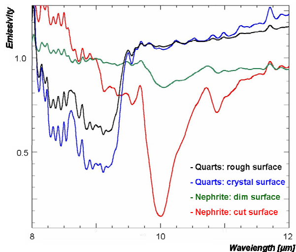
Figure 4: Emissivity of quartz and nephrite with different surfaces
